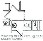
FIRST FLOOR PLAN OPTIONS
